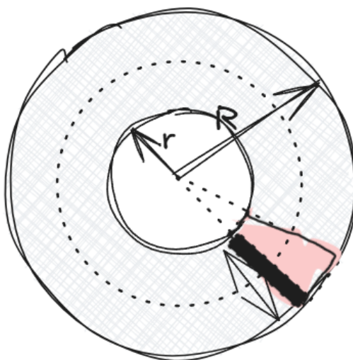
FIGURE 1.1: Calculating the area of an annulus by sweeping a line segment.
