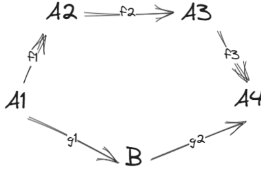
FIGURE 2.1: Mapping diagram that demonstrates f and g .
